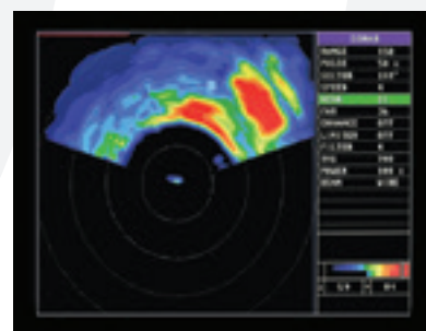
Searchlight Mode showing soft bottom and hard reef to starboard.
