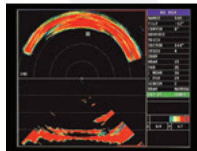
HD860 bottom typing dual beam showing hard bottom reef that could tear up a net.
